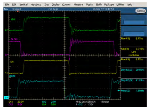
Figure 14. Gate drive and switching node fsw=1.5MHz, Io=7A
